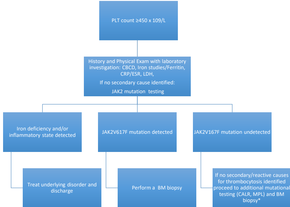
Figure 1. Diagnostic Algorithm
